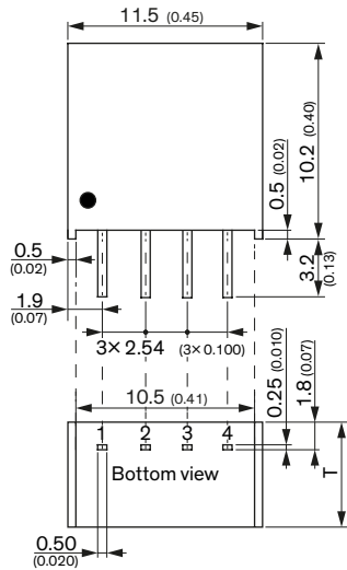
T: 6.1 (0.24) for 3.3Vin & 5Vin & 12Vin Models T: 7.1 (0.28) for 24Vin Models
