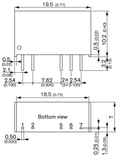
T: 6.1 (0.24) for 5 Vin & 12 Vin Models T: 7.1 (0.28) for 24 Vin Models
